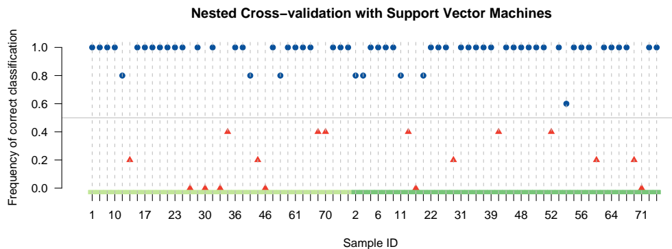
Figure 3: Visualization of the vote matrix. Samples that are misclassified most of the time are plotted in red triangles, the others in blue dots. The light green and dark green horizontal bars represent the two disease groups.
