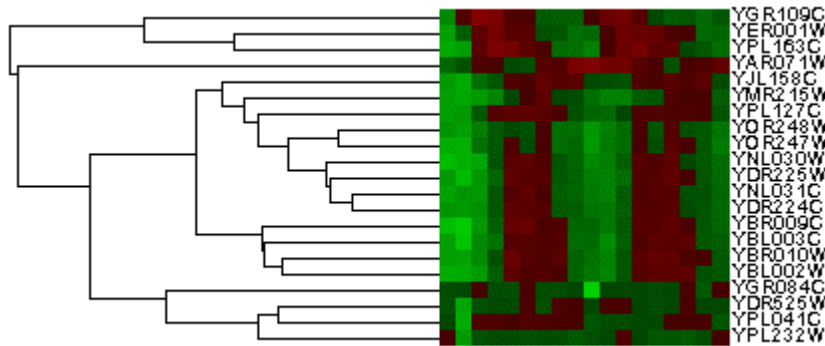
Cluster dendrogram
